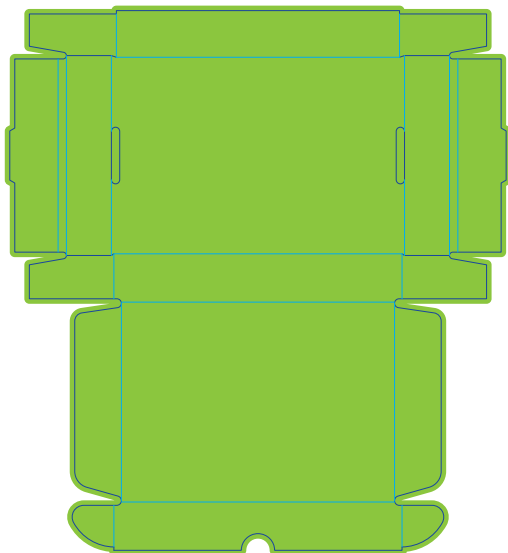
Type 1 - 164 x 28 x 120 mm (BxHxD)
