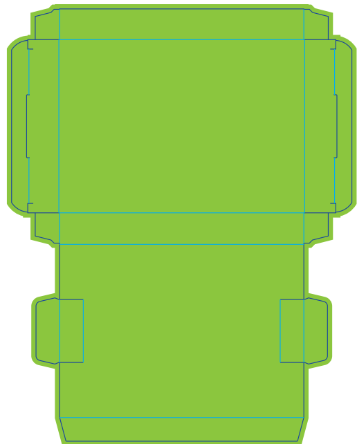
Type 2 - 155 x 20 x 110 mm (BxHxD)
